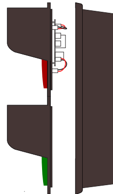
Replaceable Circuit Board Assembly
