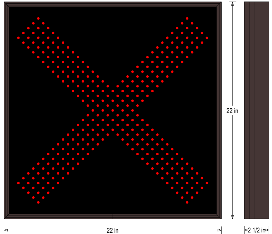
Frame Detail
