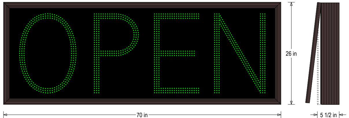
Frame Detail
