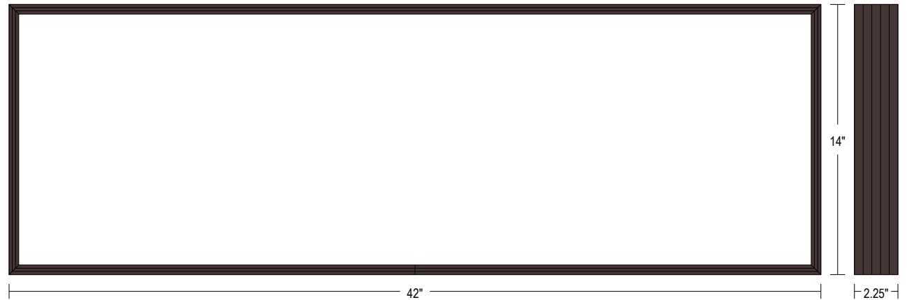
Frame Detail
