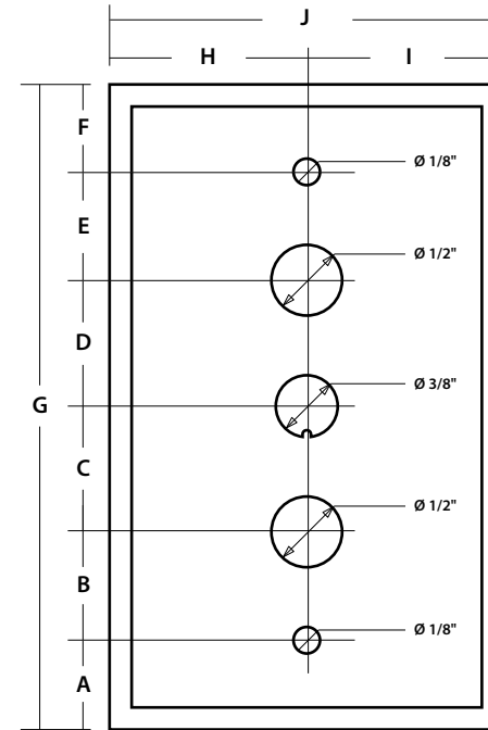
Single Gang Switch Plate
