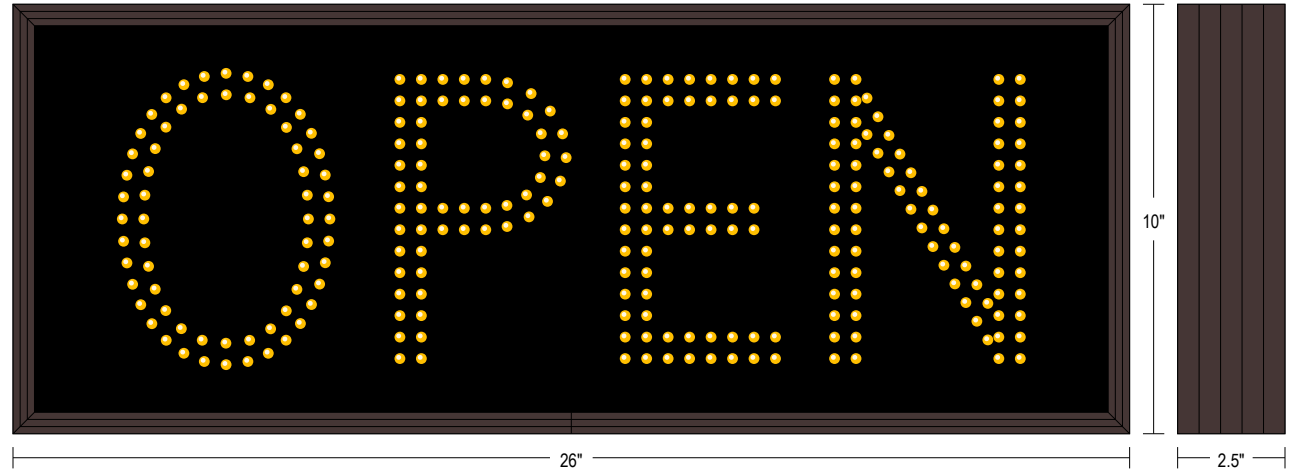
Frame Detail
