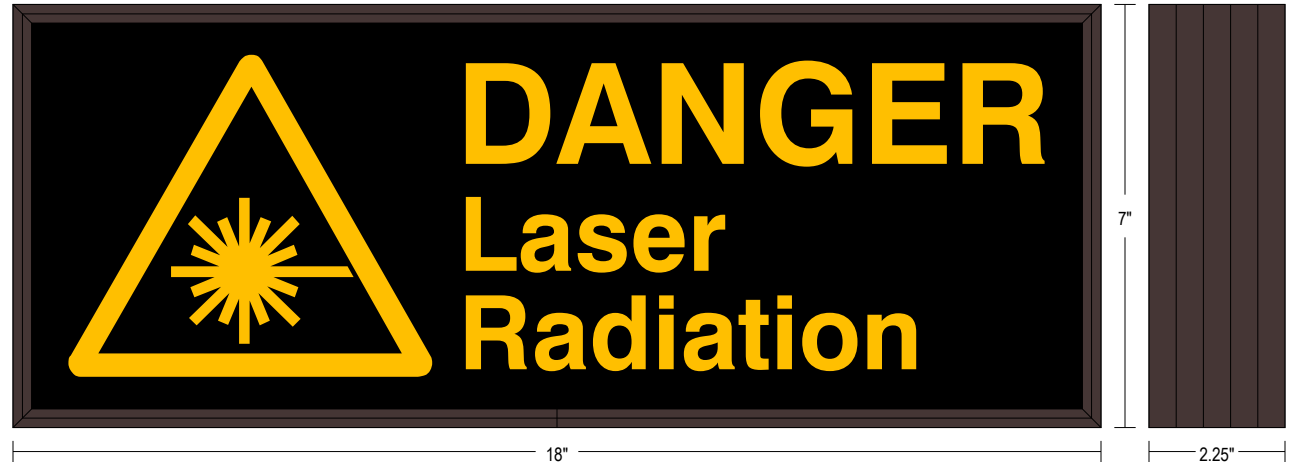
Frame Detail
