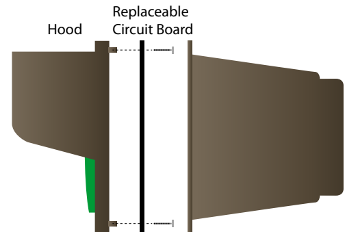
(8) #6 Stainless Steel Hi-lo screws
